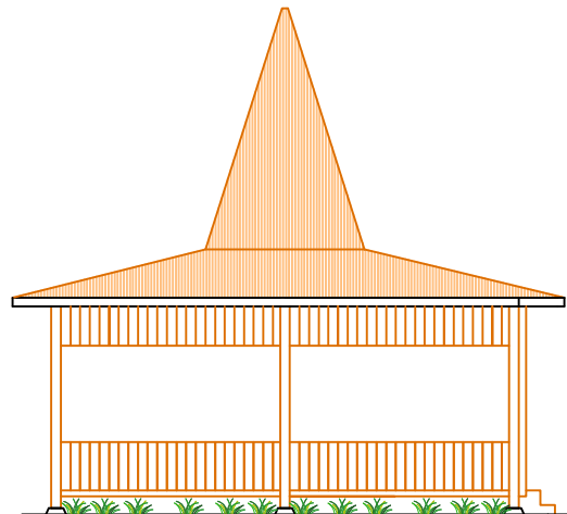
TAMPAK SAMPING KIRI
