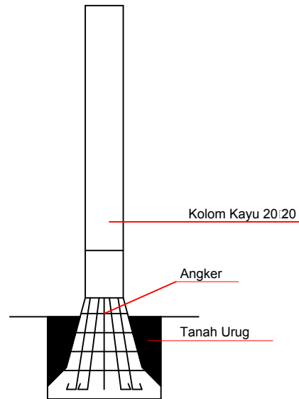
DETAIL PONDASI UMPAK
