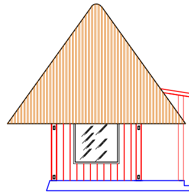
TAMPAK SAMPING KIRI SKALA 1:100
