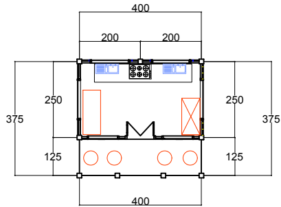
DAPUR RESTAURANT SKALA 1:100
