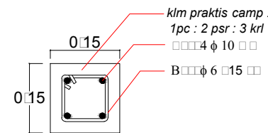
DETAIL KLM PRAKTIS
