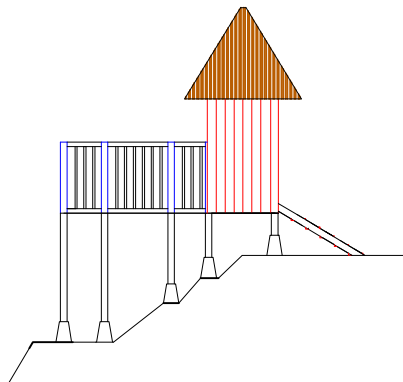
TAMPAK SAMPING SKALA 1:100
